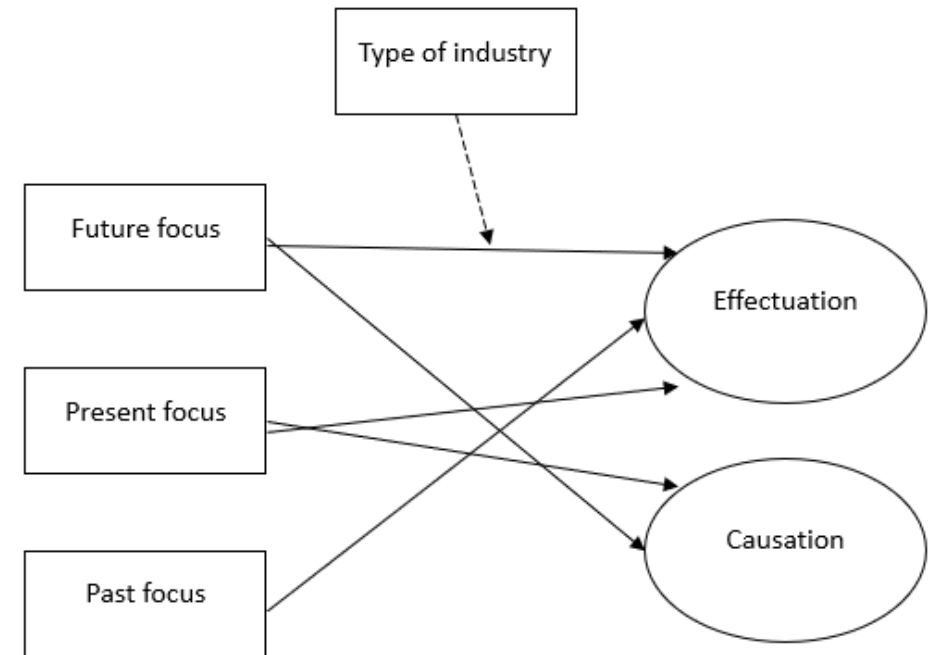
Theoretical model
